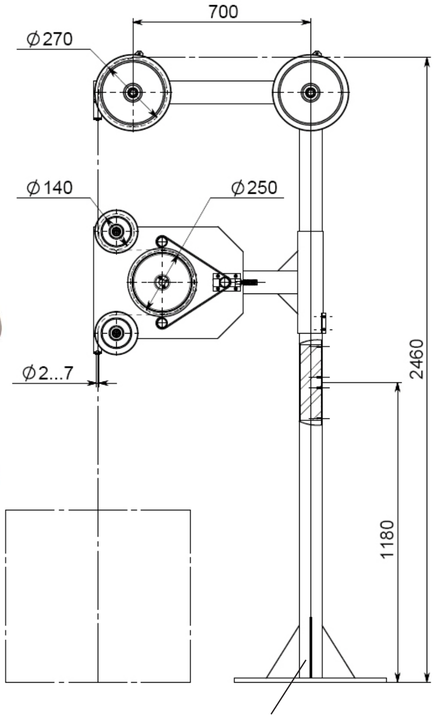
Vertical pay-off stand
